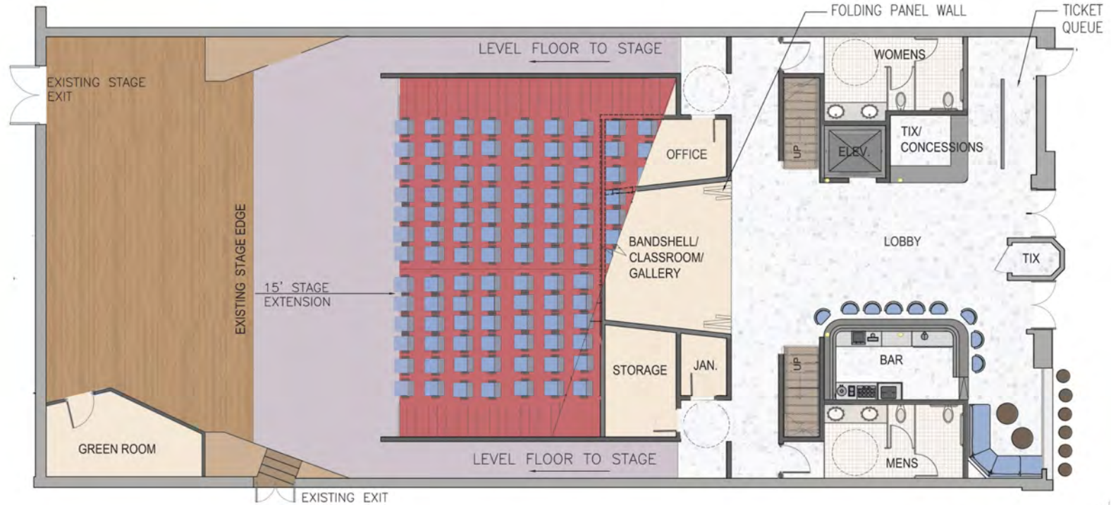
MAIN LEVEL PLAN
